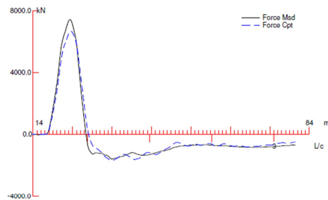
10Ton Hammer Impact
