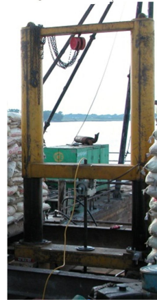
Penetrometer
